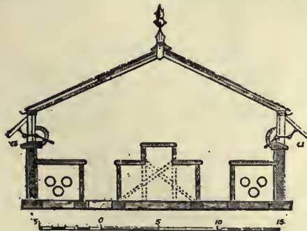
FIG. 3.—Section of Greenhouse.
